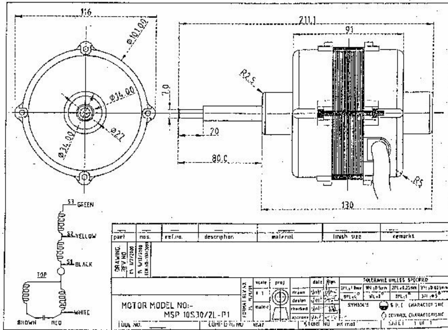
4-Pole, 1-phase, CSCR MOTOR (DIA. 100)
